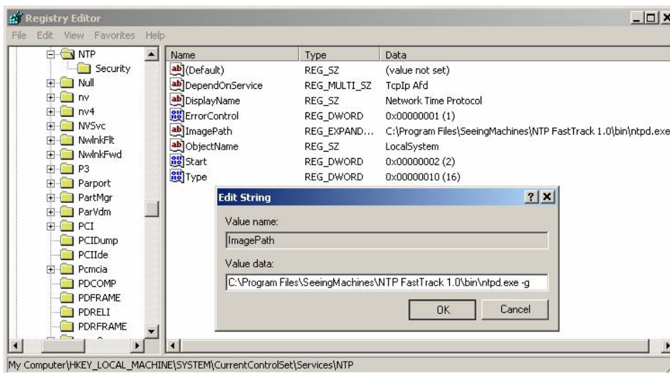
Figure 9 – Editing the registry to override the 1000 second sanity limit
