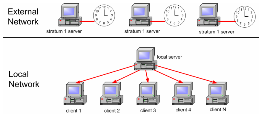
Figure 5 – Clients connected to an undisciplined server that does not reference time from other servers.
