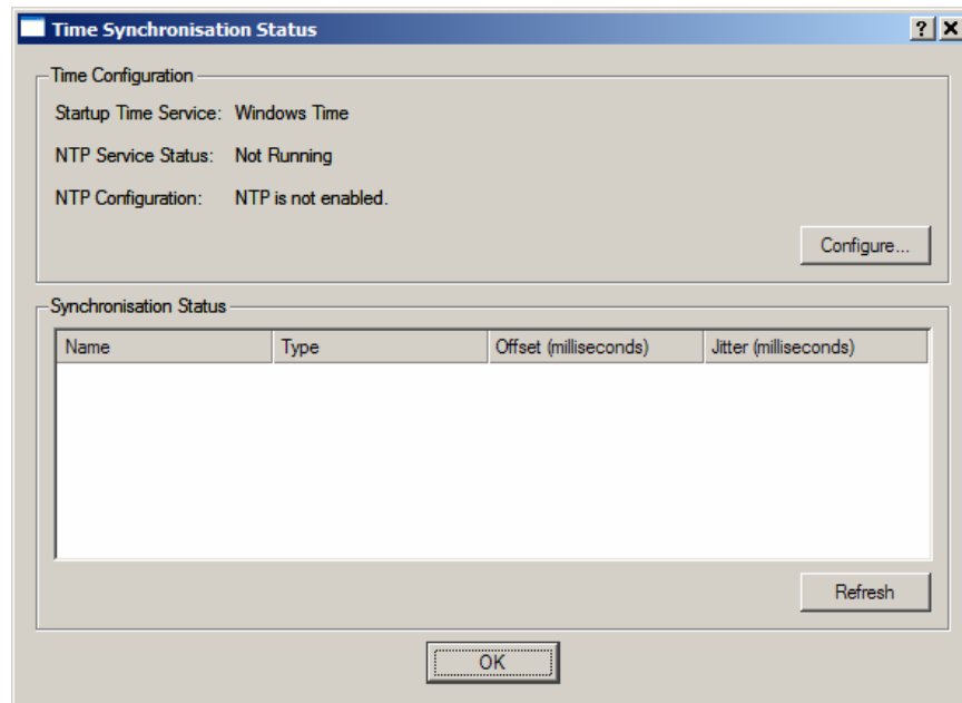
Figure 6 – The ntpstatus application
